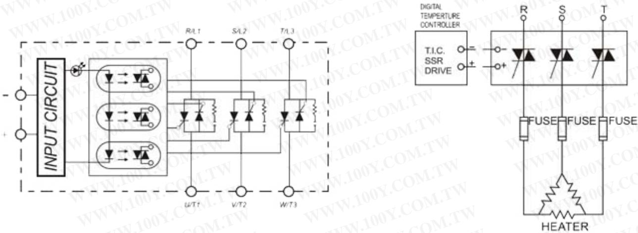
EQUIVALENT CIRCUIT
