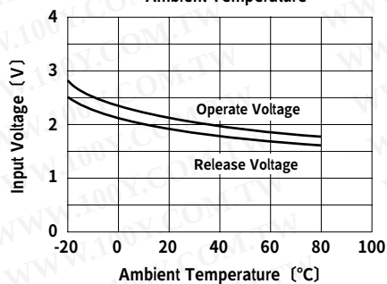
Input Characteristics VS Ambient Temperature
