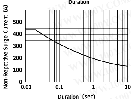
Peak Surge Current VS. Duration
