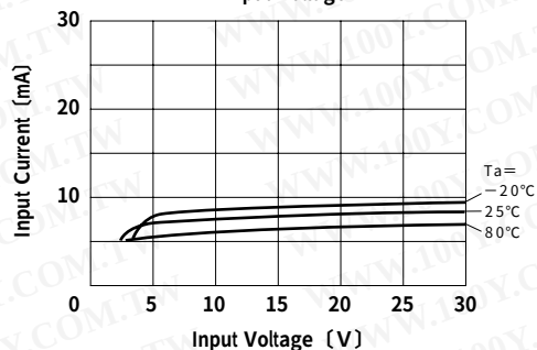
Input Current VS. Input Voltage
