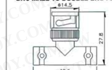
B-7077 BNC MALE TO DOUBLE BNC FEMALE
