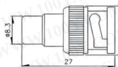
B-7056 BNC MALE TO RCA FEMALE
