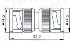
B-7046 DOUBLE BNC MALE
