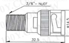
B-7050 BNC MALE TO F FEMALE
