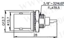
B-7031 BNC FEMALE BULKHEAD
