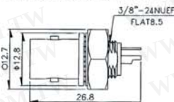
B-7035 BNC FEMALE ISOLATED GROUND BULKHEAD
