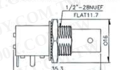
B-7044 BNC FEMALE RIGHT ANGLE PANEL MOUNT
