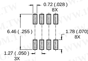
RECOMMENDED FOOTPRINT
