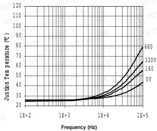
Figure 8. IR2133J Junction Temperature vs Frequency Driving (IRGPC30KD2) R_{gate} = 5.1\Omega @ V_{cc} = 15V
