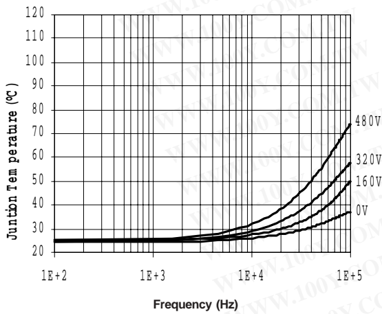
Figure 7. IR2133J Junction Temperature vs Frequency Driving (IRGPC20KD2) R_{gate} = 5.1\Omega @ V_{cc} = 15V
