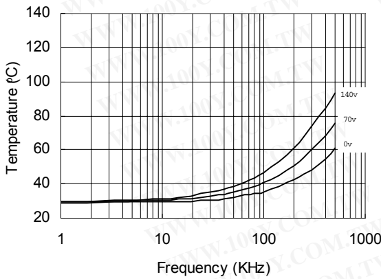
Figure 23. IR2181 vs. Frequency (IRFBC40), R_{gate} = 15\Omega, V_{CC} = 15V
