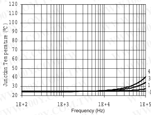
Figure 55. IR2130J/IR2132J T J vs. Frequency (IRGPC20KD2) R GATE = 33Ω, V CC = 15V
