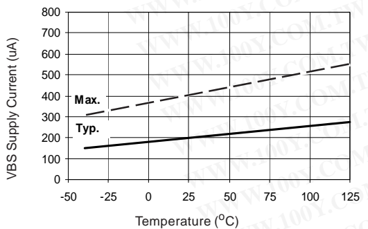
Figure 23A VBS Supply Current vs Temperature
