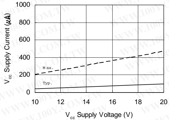
Figure 14B. V_{cc} Supply Current vs. Supply Voltage
