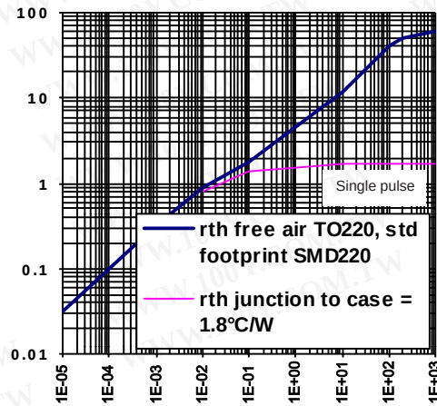
Figure 16 - Transient Thermal Imped. (°C/W) Vs Time (s) - IPS0151/IPS01S
