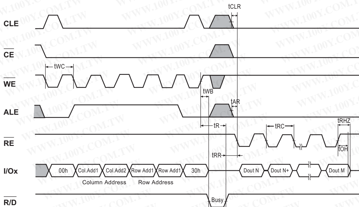
Figure 11: Read1 Operation intercepted by CE#
