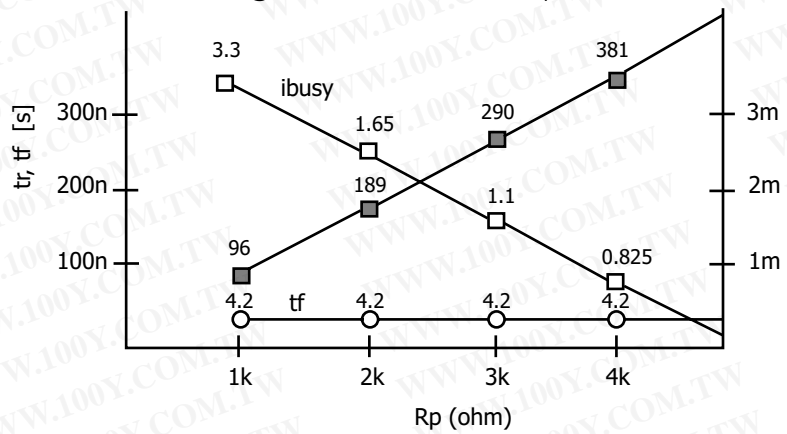
Fig. Rp vs tr, tf & Rp vs ibusy
