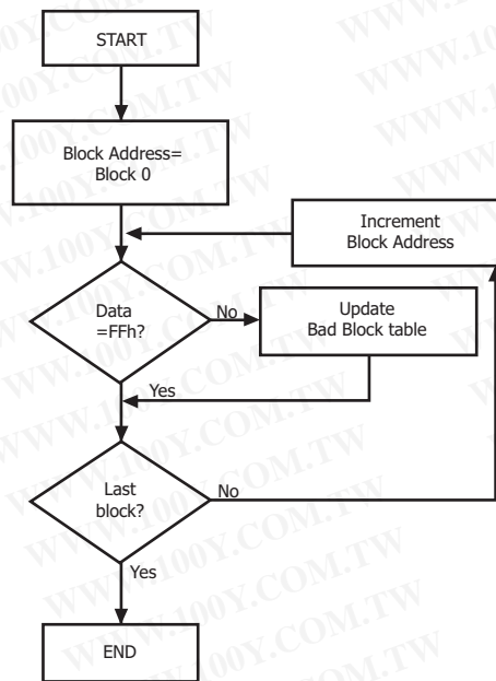
Figure 28: Bad Block Management Flowchart
