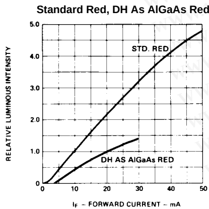
Figure 3. Relative luminous intensity vs. forward current (non-resistor lamp).
