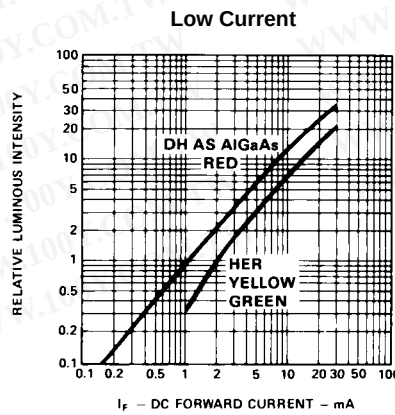
Figure 3. Relative luminous intensity vs. forward current (non-resistor lamp).
