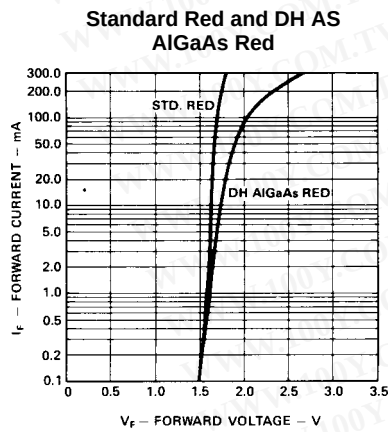
Figure 2. Forward current vs. forward voltage (non-resistor lamp).
