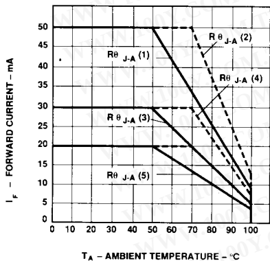
Figure 5. Maximum forward dc current vs. ambient temperature. Derating based on T j MAX = 110°C (non-resistor lamps).
