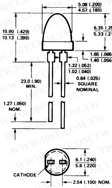
PACKAGE OUTLINE "B" HLMP-3390, -3490, -3590
