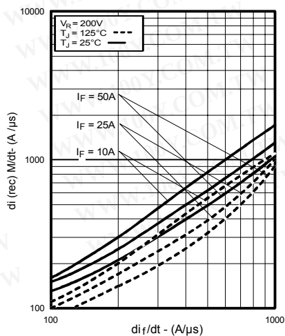
Fig. 8 - Typical di_{(rec)}M/dt vs. di/dt
