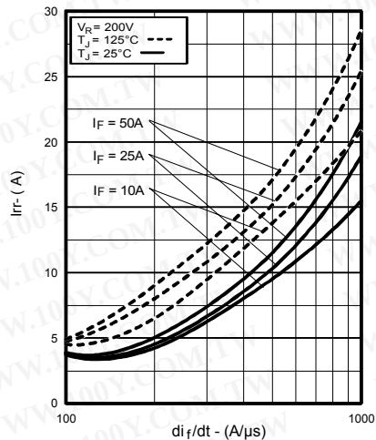
Fig. 6 - Typical Recovery Current vs. di/dt
