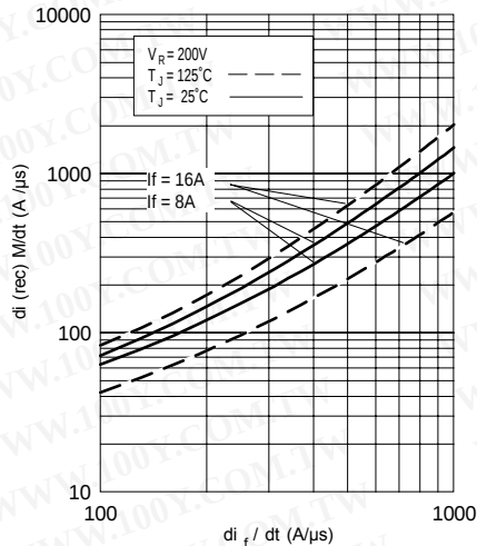
Fig. 8 - Typical di_{(rec)}M/dt vs. di/dt , (per Leg)
