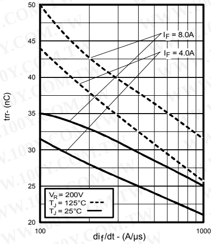
Fig. 5 - Typical Reverse Recovery vs. di/dt
