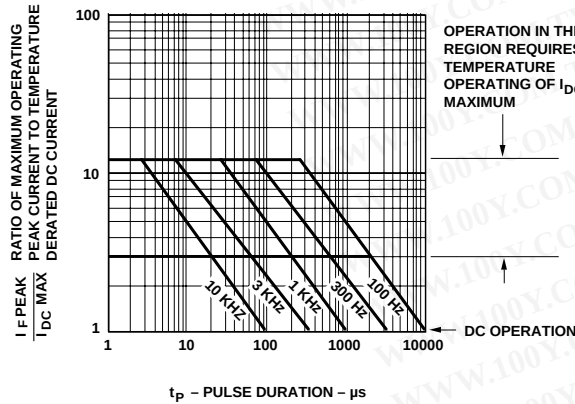
Figure 8. Allowable Peak Current vs. Pulse Duration - Green.
