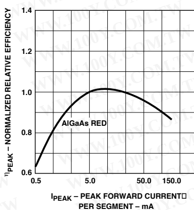
Figure 6. Relative Efficiency (Luminous Intensity per Unit Current) vs. Peak Current.
