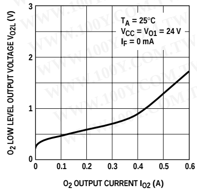
Figure 30. Typical Low Level Output 2 Voltage vs. Output 2 Current, HCPL-3101.
