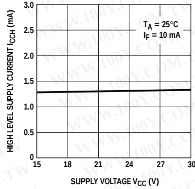
Figure 33. Typical High Level Supply Current vs. Supply Voltage, HCPL-3100.
