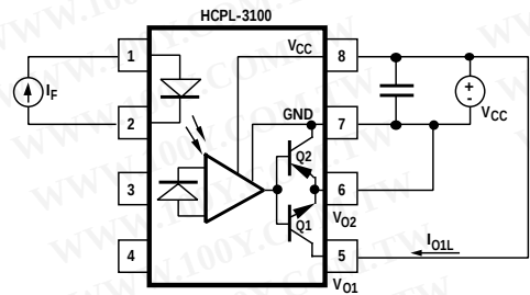
Figure 5. Test Circuit for Leakage Current I_{O1L} .
