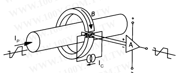
圖1. Representation of the electrical parameters of the Hall effect 圖2. Conversion of the primary current into an output voltage
