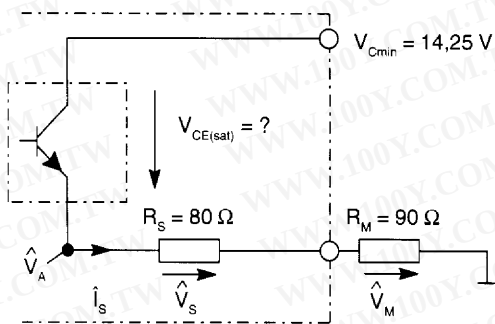
圖 8. Equivalent diagram for calculation of the available voltage V_A on the final stage of the amplifier.
