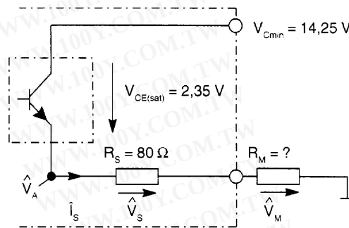
圖 9. Equivalent diagram to calculate the measuring resistance R_M
