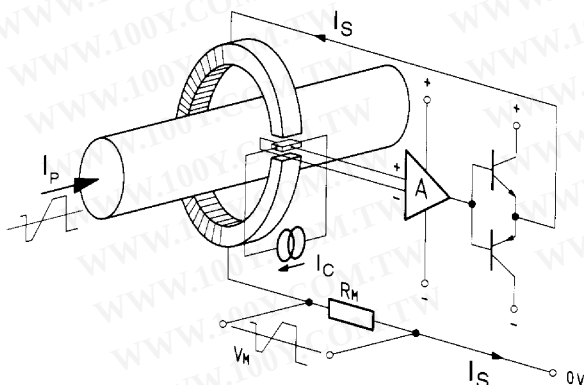
圖 6. Operating principle of the closed loop transducer
