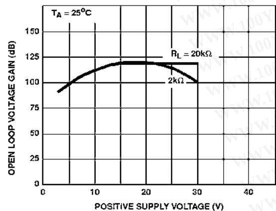
FIGURE 5. VOLTAGE GAIN vs SUPPLY VOLTAGE
