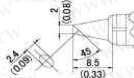
T10-C5 Shape-5C Bevel T10-CF5 ※
