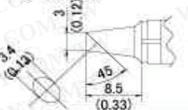
T10-C6 Shape-6C Bevel
