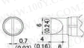
T10-K Shape-K Knife
