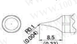
T10-KL Shape-KL Knife
