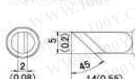
T10-LB Shape-LB Long Conical
