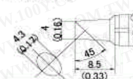
T10-D08 Shape-0.8D Chisel
