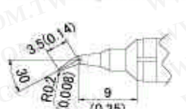
T10-KU Shape-KU Knife
