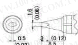
T10-D4 Shape-4D Chisel
