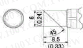
T10-D16 Shape-1.6D Chisel
