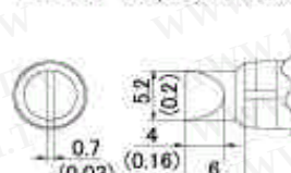
T10-J02 Shape-0.2RSB Bent
