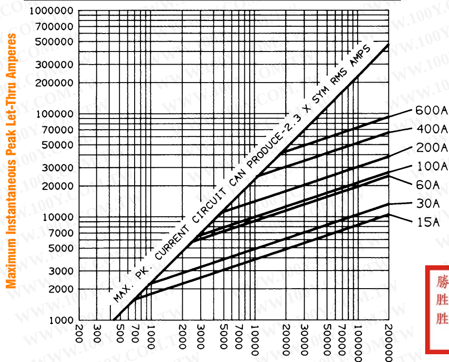
Peak Let-Thru Current Data — TR30 to 600, 250 Volts AC
