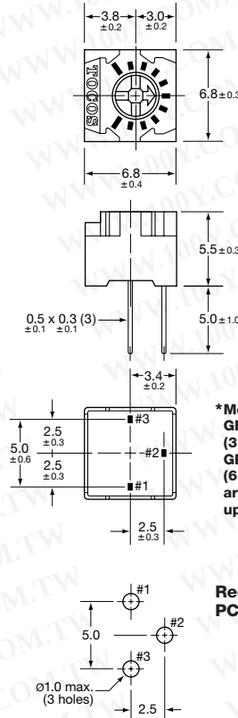
GF063U Cross-Slot, Top Adjust, U & U-LL* Terminal Styles
