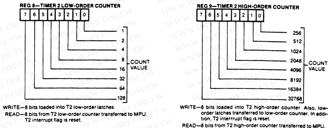
Figure 27. T2 Counter Format and Operation
