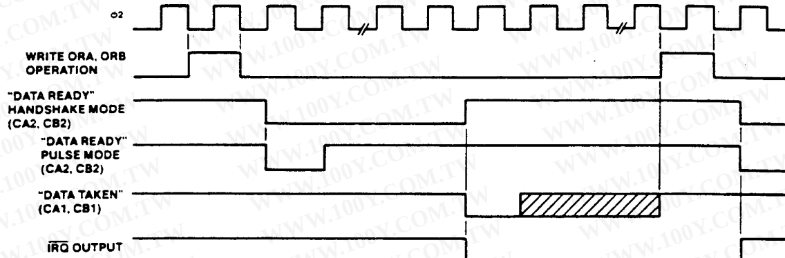
Figure 20. Write Handshake (Ports A and B)
