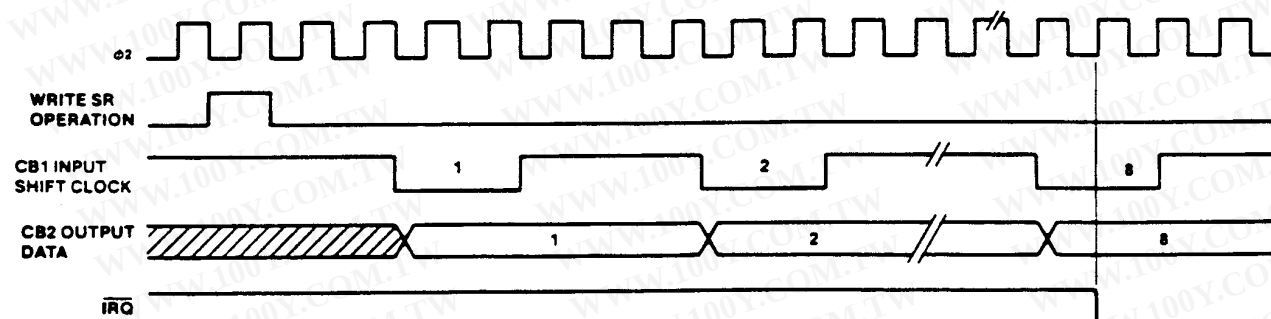
Figure 36. Shift Out—External CB1 Clock Control
