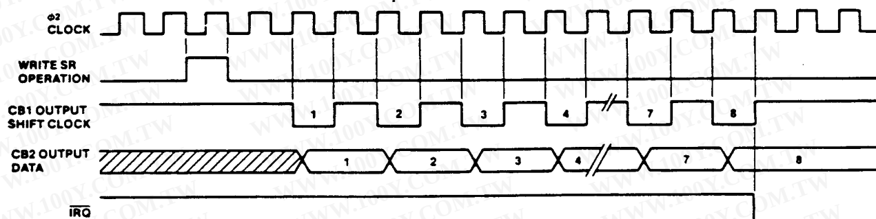
Figure 35. Shift Out— \phi 2 Control
