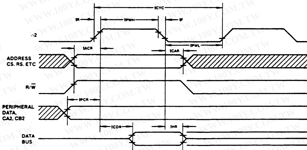
Figure 2. Read Timing
