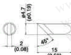
T12-KR SHAPE-KR
