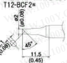
T12-BC2 SHAPE-2BC
