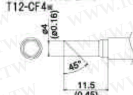
T12-C4 SHAPE-4C
