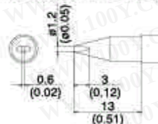
T12-DL12 SHAPE-1.2DL
