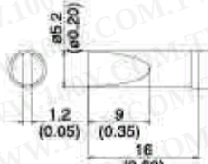
T12-DL52 SHAPE-5.2DL
