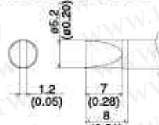
T12-DL32 SHAPE-3.2DL
