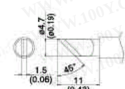
T12-KL SHAPE-KL
