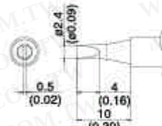
T12-DL08 SHAPE-0.8DL
