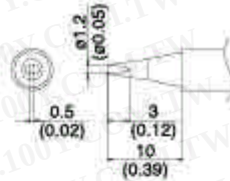
T12-D4 SHAPE-4D
