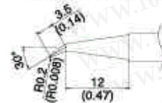
T12-J02 SHAPE-0.2J
