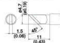
T12-KR SHAPE-KR
