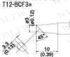
T12-BC3 SHAPE-3BC
