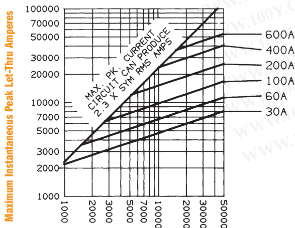
Peak Let-Thru Current Data – OT, OTN & OTS30 to 600, 250 and 600 Volts AC
