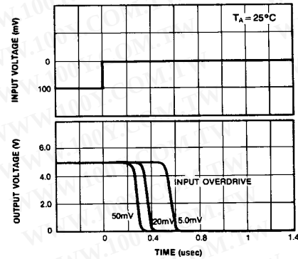
Figure 4. Response Time for Various Input Overdrive-Negative Transition
