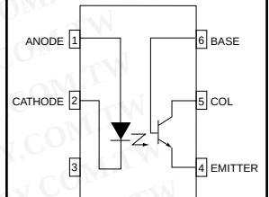
SCHEMATIC
