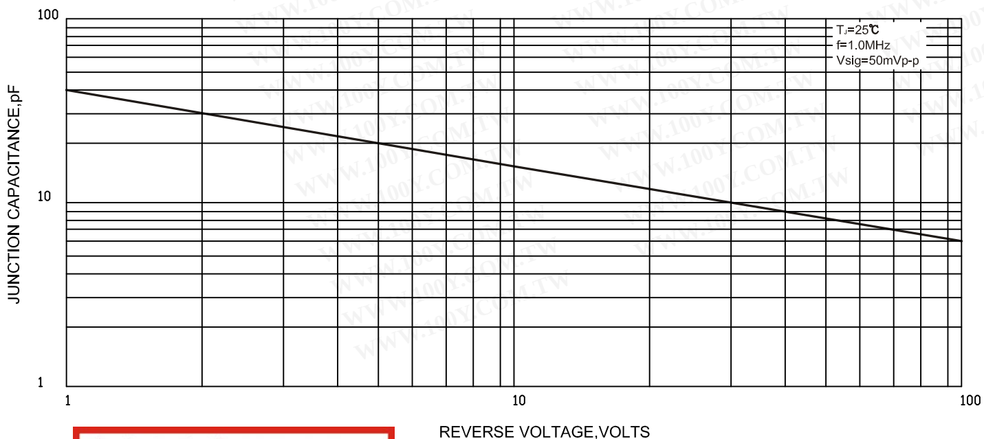
FIG.5-TYPICAL JUNCTION CAPACITANCE
