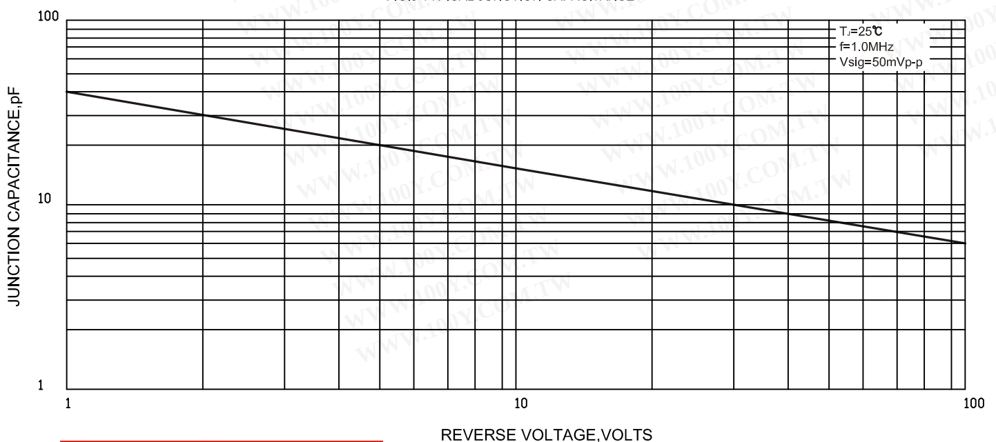
FIG.5-TYPICAL JUNCTION CAPACITANCE
