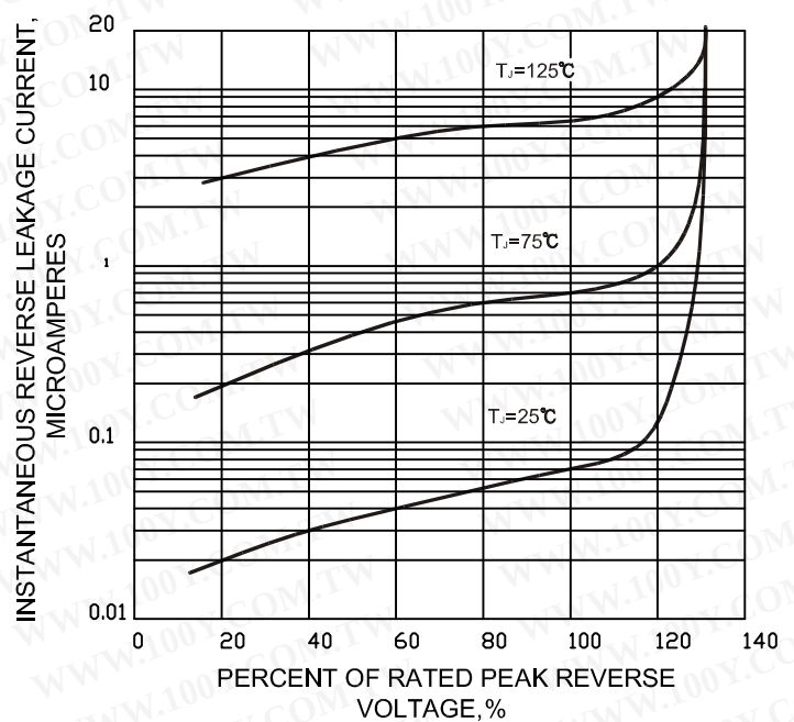
FIG.4-TYPICAL REVERSE CHARACTERISTICS
