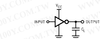
FIGURE 1. AC Test Circuit
