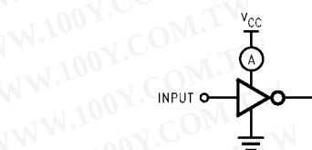
FIGURE 2. I CCD Test Circuit
