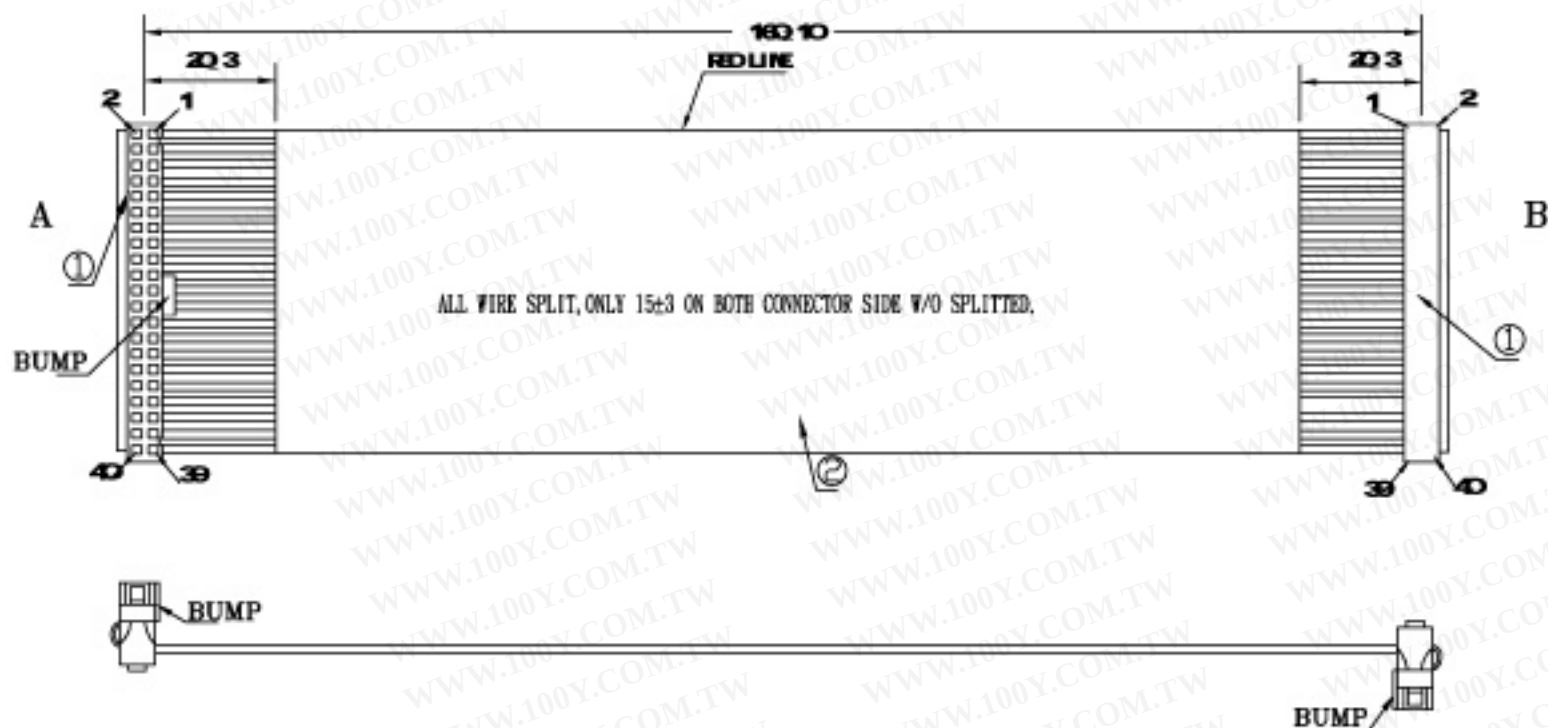
PIN ASSIGNMENT
