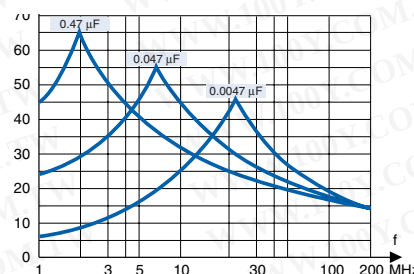
Suppression versus frequency. Typical values.
