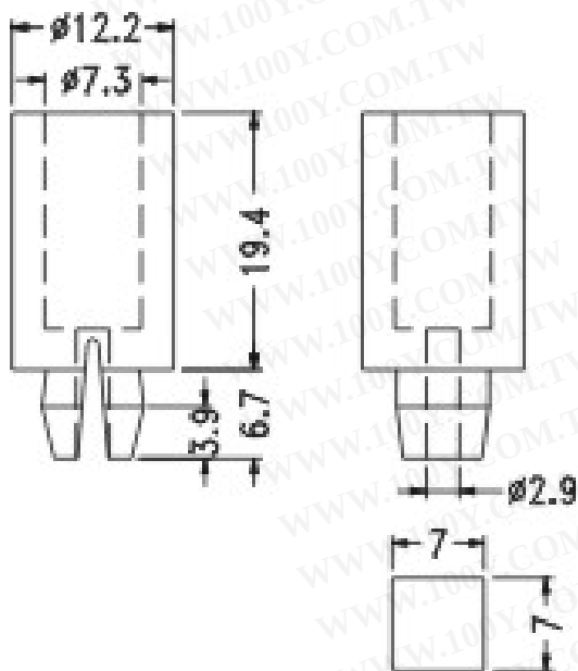
MOUNTING HOLE
