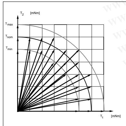
Figure 8b. An example of accessible positions with a given torque deviation/fullstep. Note that 1:st μstep sets highest resolution. Data points are exaggerated for illustration purpose. TNom = code 127.
