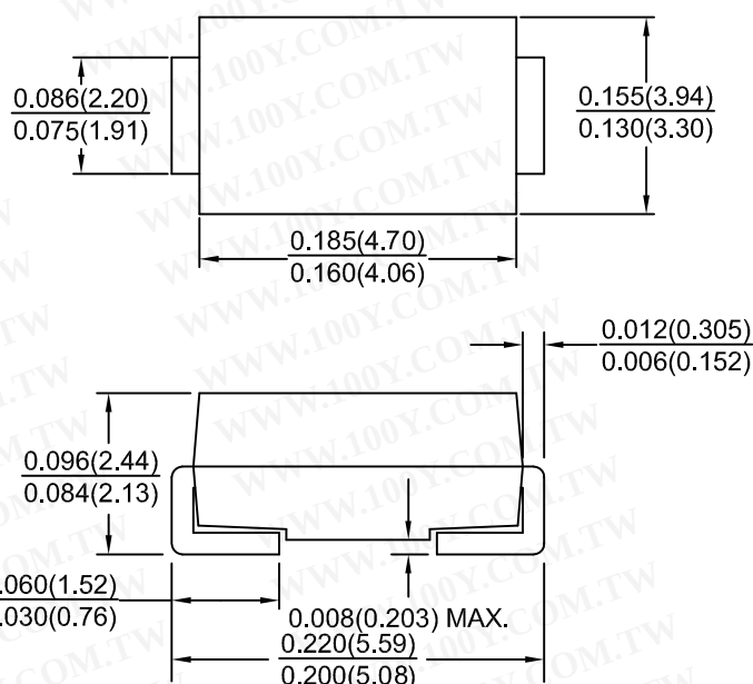
SMB/DO-214AA
