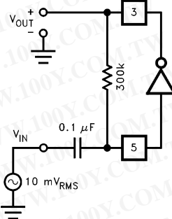
Test Circuit 1
