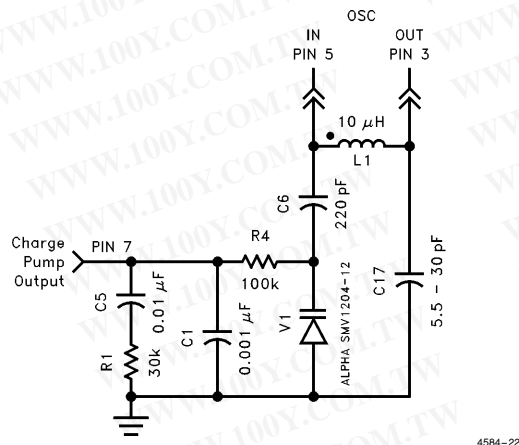
(3) LC Tank
