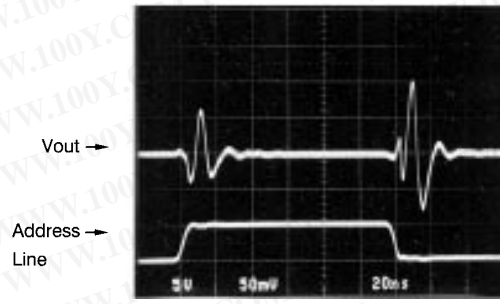
Channel-to-Channel Switching Glitch
