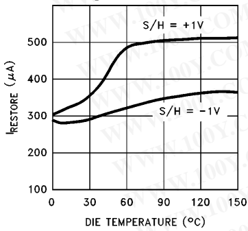
Restoring Current vs Temperature
