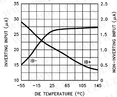
Amplifier Input Current vs Die Temperature
