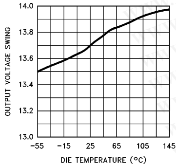
Amplifier Output Voltage vs Die Temperature; V_S = \pm 15V
