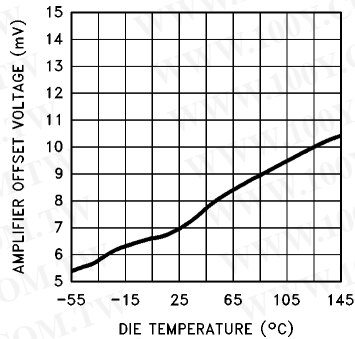
Amplifier Offset Voltage vs Die Temperature
