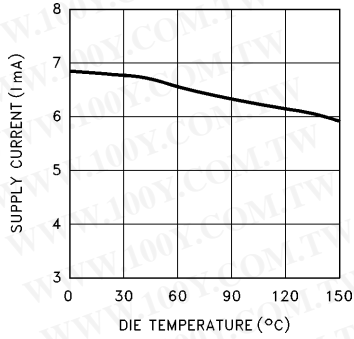
Supply Current vs Temperature V_S = \pm 15V
