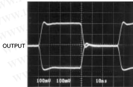
EL2140 Small Signal Response (Note 1)
