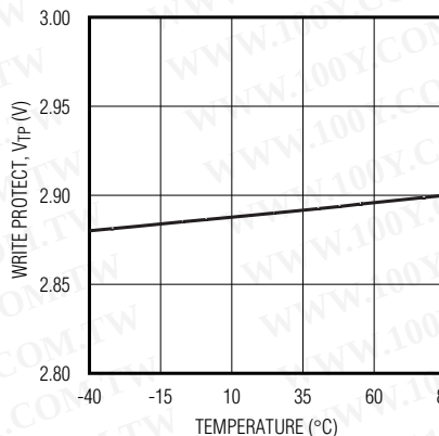
WRITE PROTECTION VOLTAGE vs. TEMPERATURE
