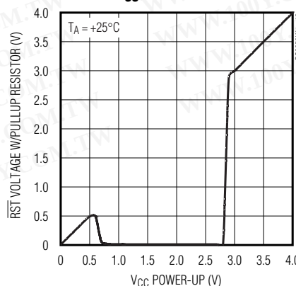
RST VOLTAGE vs. V CC DURING POWER-UP
