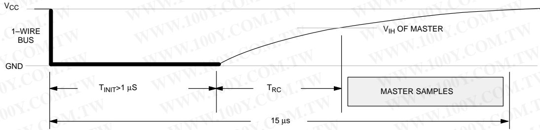
DETAILED MASTER READ "1" TIMING Figure 13
