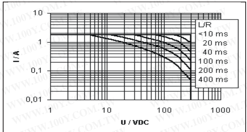
Derating curve for inductive loads.
