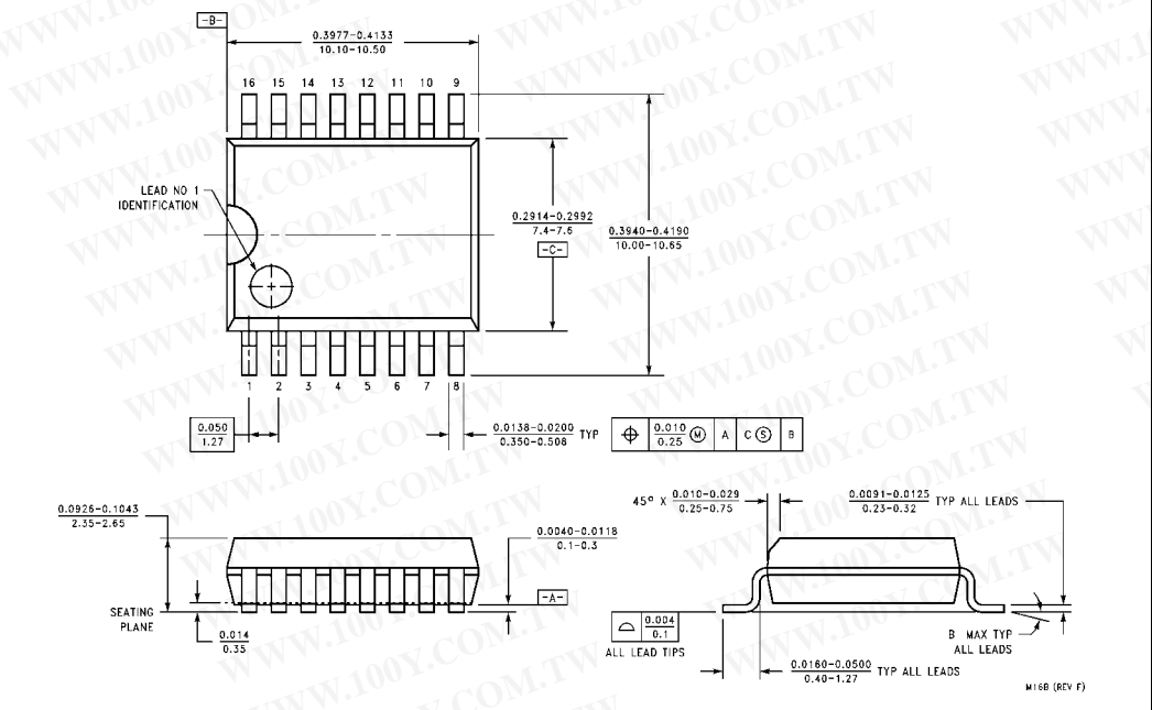
16-Lead Small Outline Integrated Circuit (SOIC), JEDEC MS-013, 0.300" Wide Body Package Number M16B
