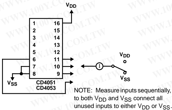
FIGURE 19. INPUT CURRENT
