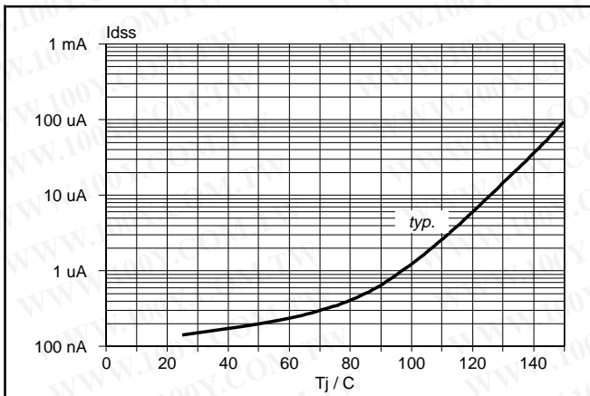
Fig.36. Typical off-state leakage current. I_{DSS} = f(T_j) ; Conditions: V_{DS} = 40\text{ V} ; V_{IS} = 0\text{ V} .
