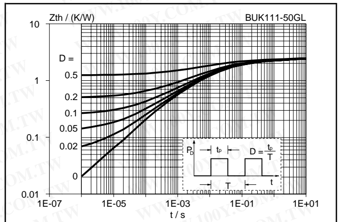
Fig.38. Transient thermal impedance. Z_{th\ j-mb} = f(t) ; parameter D = t_p/T
