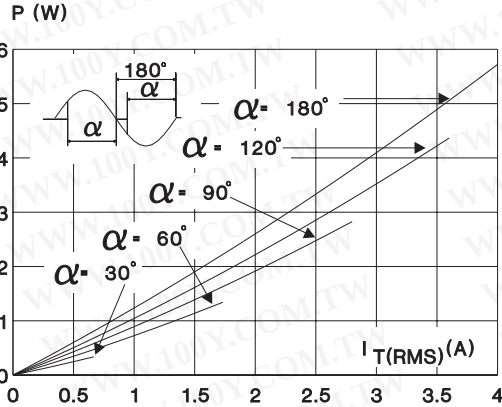
Fig. 1: Maximum RMS power dissipation versus RMS on-state current ( F = 50\text{Hz} ). (Curves are cut off by (di/dt)_c limitation)
