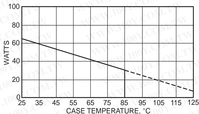
Figure 2: Power Derating, Each Active FET
