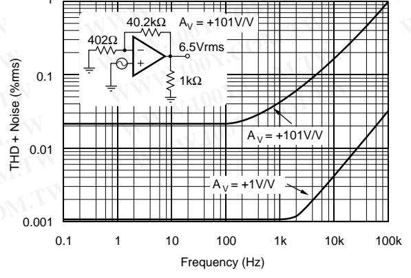
TOTAL HARMONIC DISTORTION vs FREQUENCY
